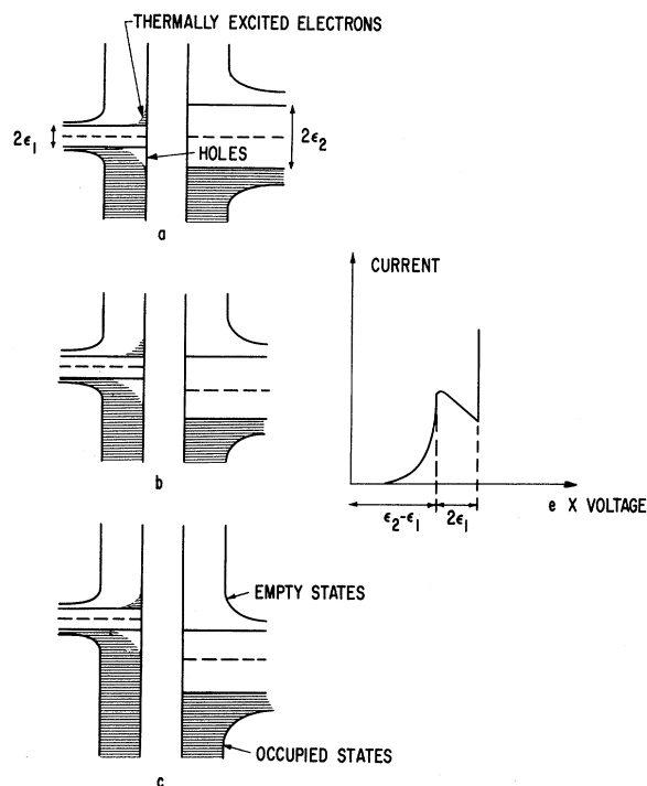
FIG. 1. Analysis of the current-voltage characteristic of two superconductors separated by a thin film. (a) The two superconductors with no voltage applied. Thermally excited electrons and holes are shown for the smaller gap, while for the larger gap there will be relatively few thermally excited electrons. (b) When a voltage is applied, a current will flow and will increase with voltage, because more and more of the thermally excited electrons in the left-hand superconductor are raised above the forbidden gap in the right-hand superconductor, and can tunnel. When the applied voltage corresponds to half the difference of the two energy gaps, \epsilon_2 - \epsilon_1 , it has become energetically possible for all the thermally excited electrons to tunnel through the film. (c) When the voltage is increased further, only the same number of electrons can tunnel, and since they now face a less favorable (lower) density of states, the current will decrease. Finally, when a voltage greater than half the sum of the two energy gaps, \epsilon_2 + \epsilon_1 , is applied, the current will increase rapidly because electrons below the gap can begin to flow.
