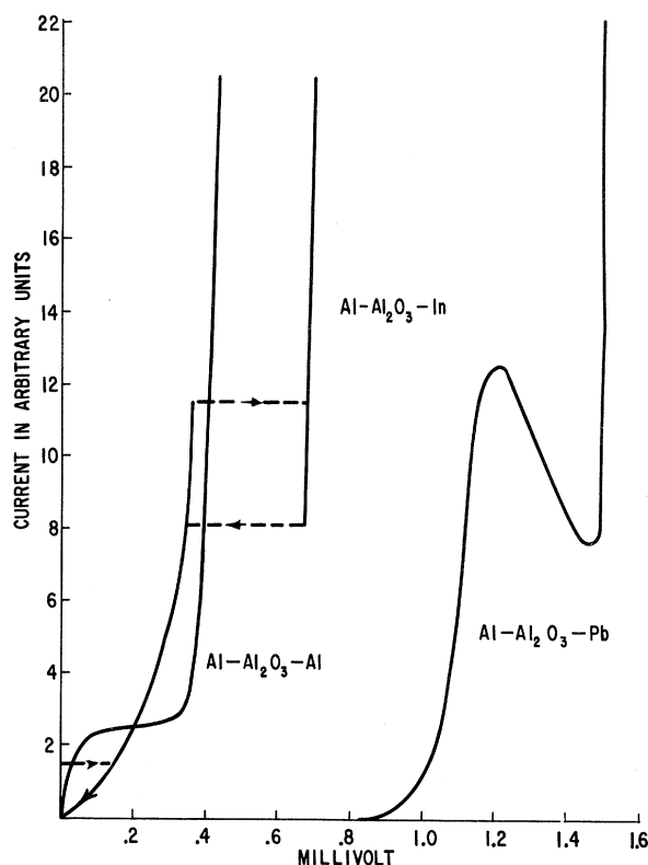
FIG. 2. Characteristic curves for tunneling between two superconductors, showing agreement with the analysis of Fig. 1. The curves Al-Al 2 O 3 -In and Al-Al 2 O 3 -Al are taken at T \sim 1.1^\circ\text{K} , while the curve Al-Al 2 O 3 -Pb is at T \sim 1.0^\circ\text{K} .
